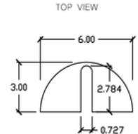
MOUNTING SLOT DETAIL SCALE 2:1 ALL DIMS NOMINAL
